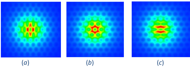
Figure 1: Dominant magnetic field distribution for each type of core. (a) yEC-CHF, (b) xEC-CHF, (c) CC-CHF
